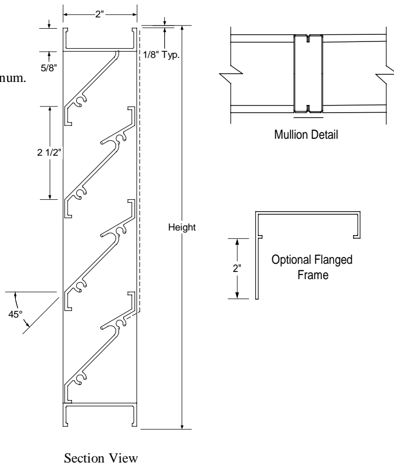
Section View
